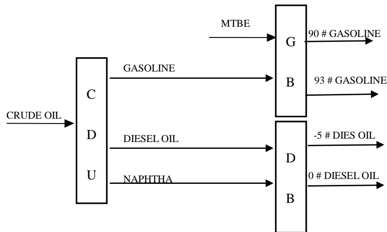
Figure 4 The configuration of example 2
